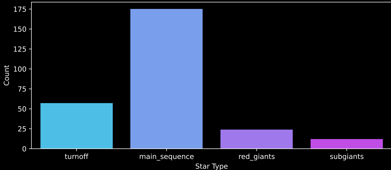
GALAH DR4 Field: [6957] Count plot of Star Type
