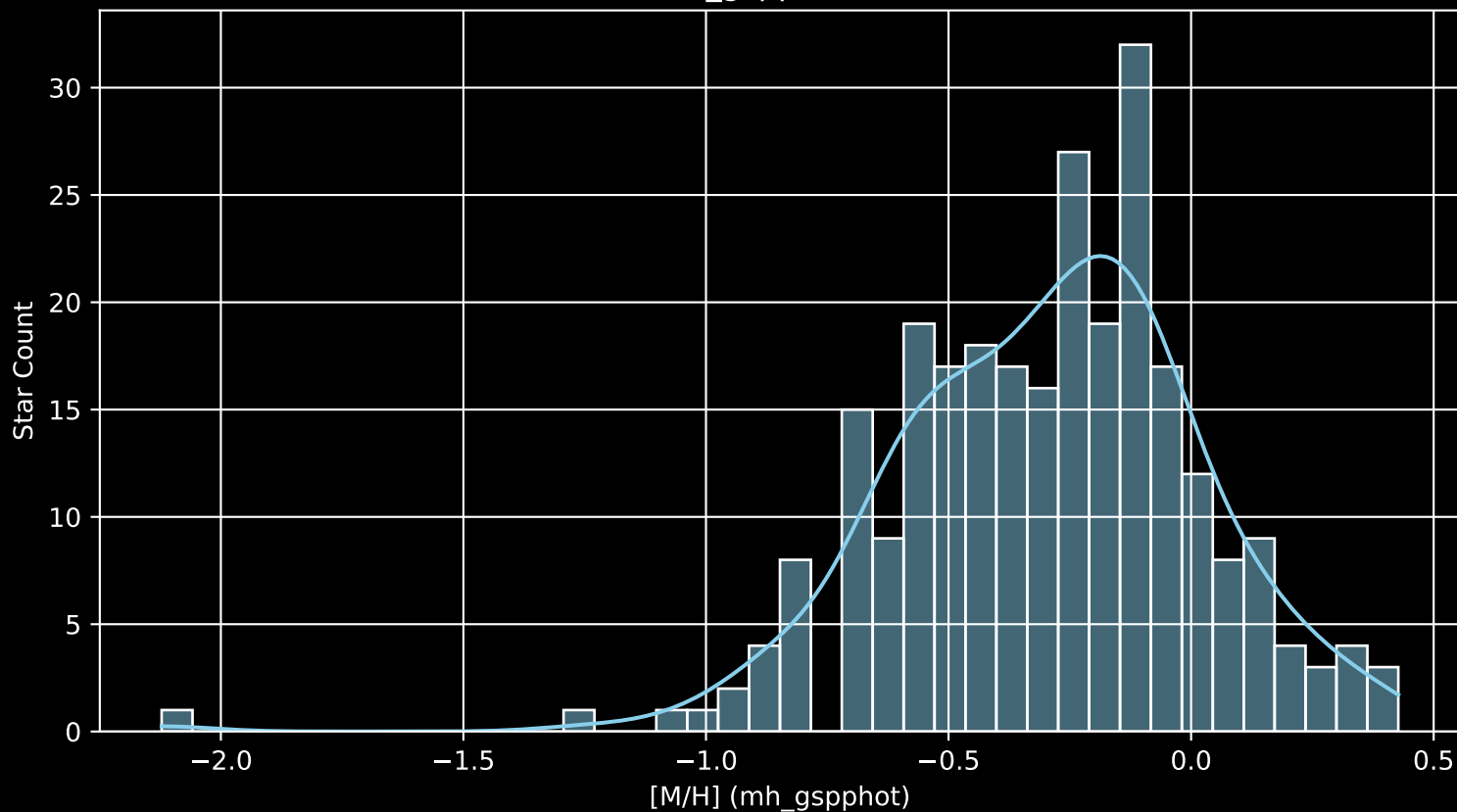
GALAH DR4 Field: [6957] [M/H] (mh_gspphot) (n= 267)
