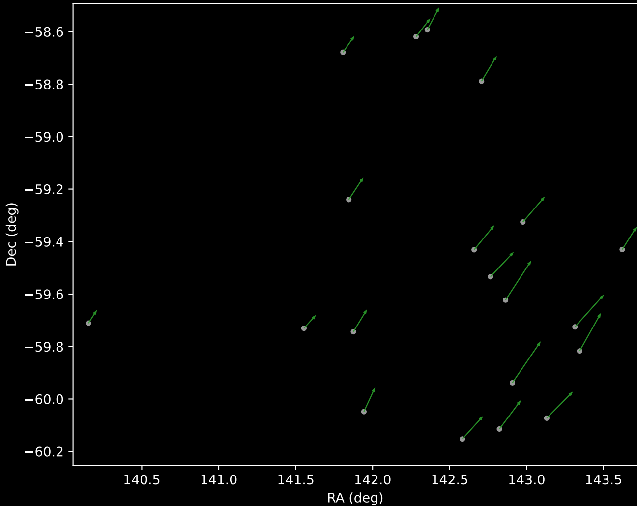
GALAH DR4 Cluster 4 Proper Motion Vectors (n=20)
