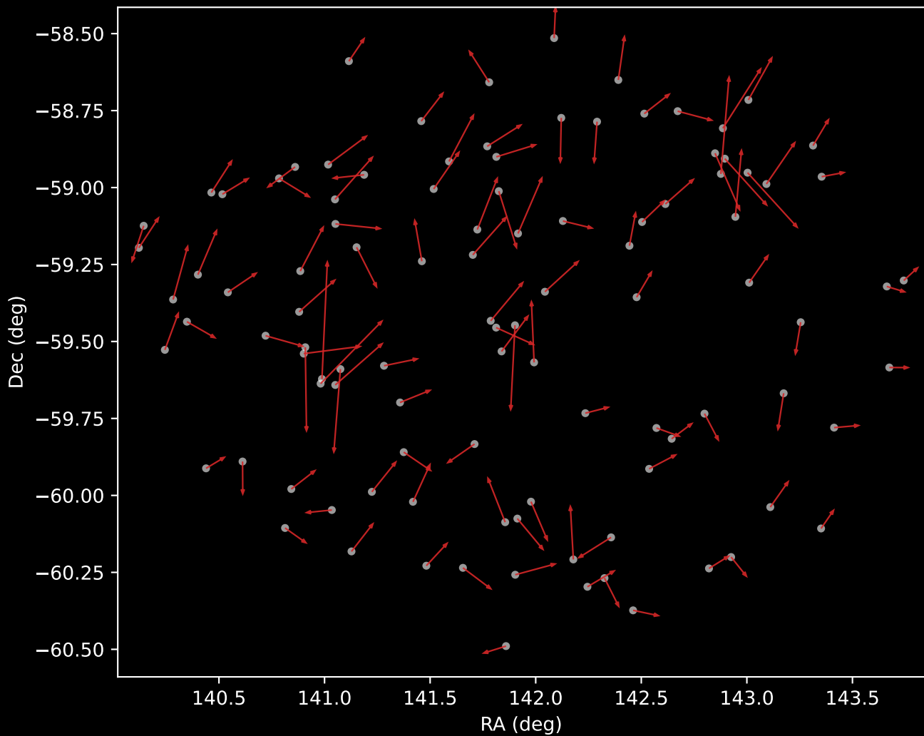
GALAH DR4 Cluster 6 Proper Motion Vectors (n=104)
