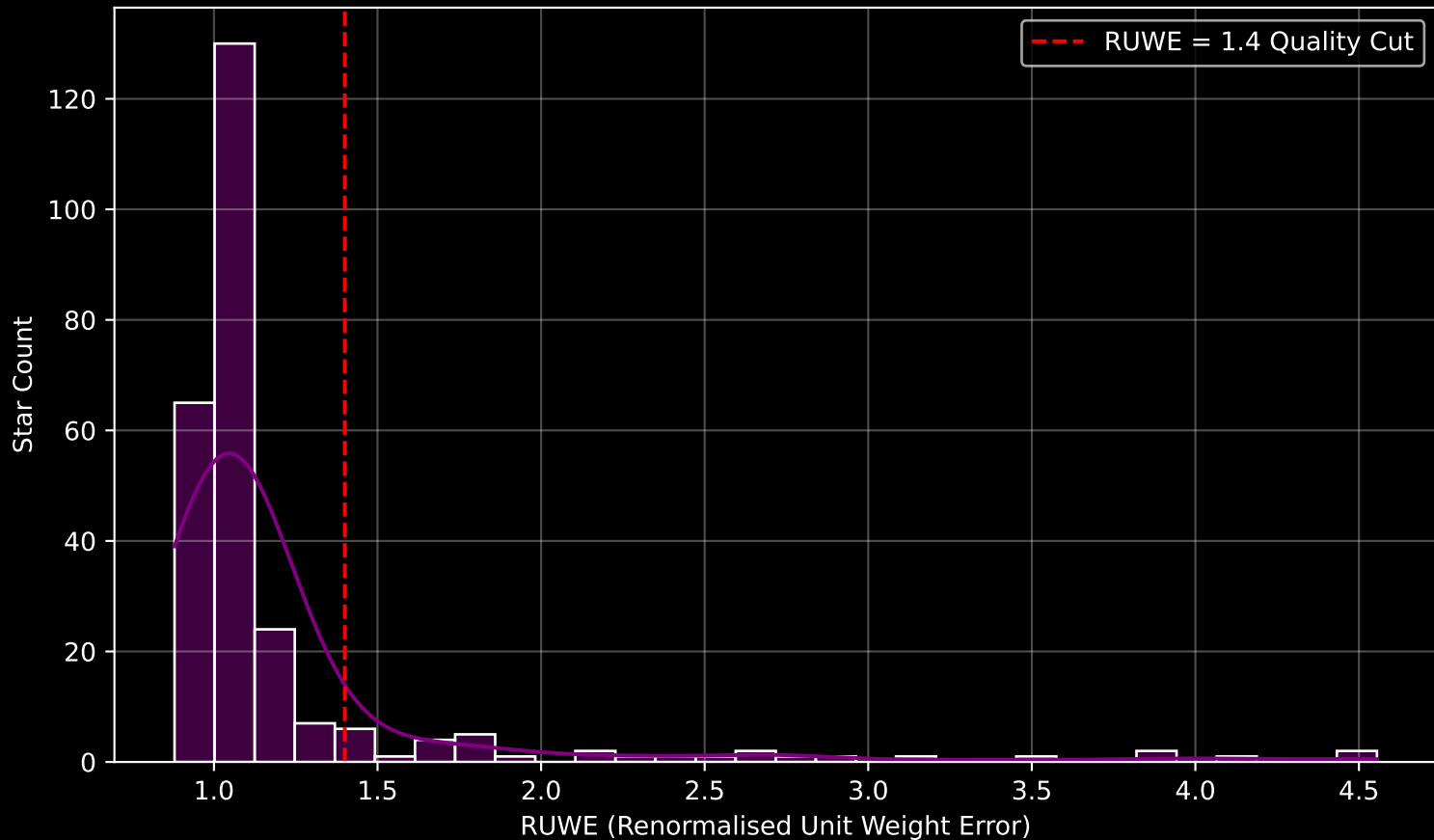
GALAH DR4 Field [6957] RUWE Distribution (n= 259)
