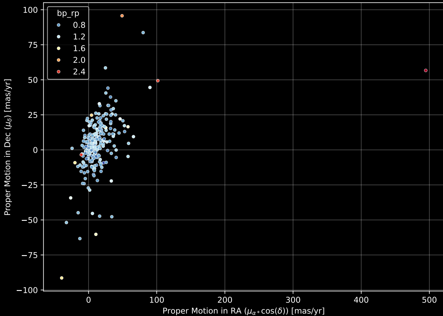
GALAH DR4 Field: [6957] Proper Motion Diagram (n= 268)
